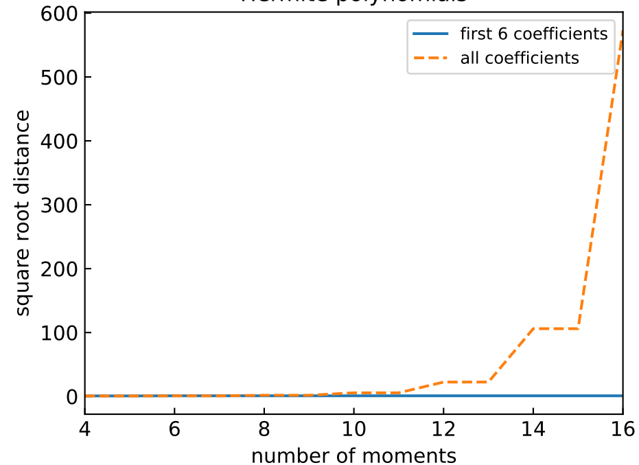
Hermite polynomials
