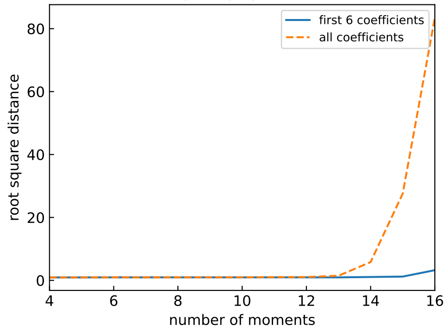
Logistic polynomials
