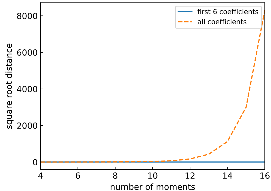
Hermite polynomials
