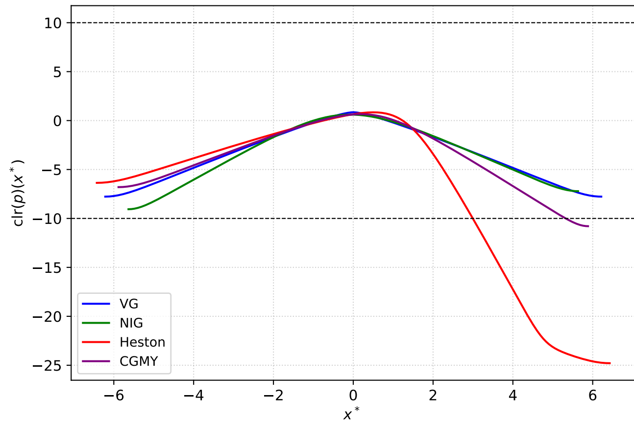
CLR of four standardized PDFs ( L=4 ), with CGMY
