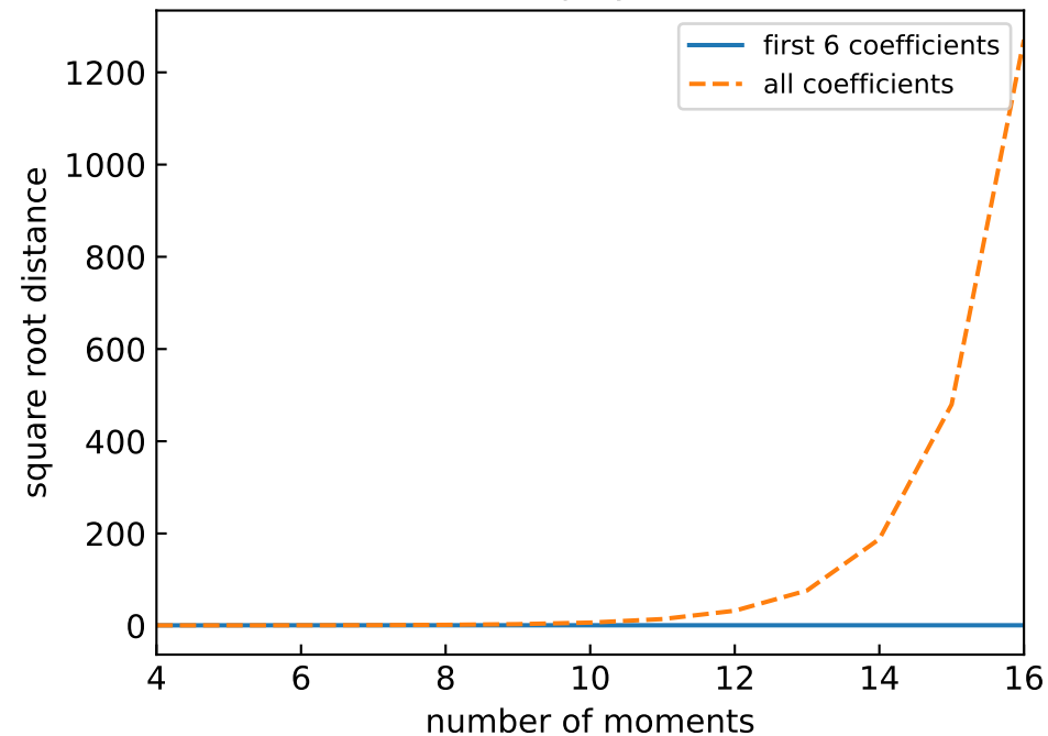
Hermite polynomials
