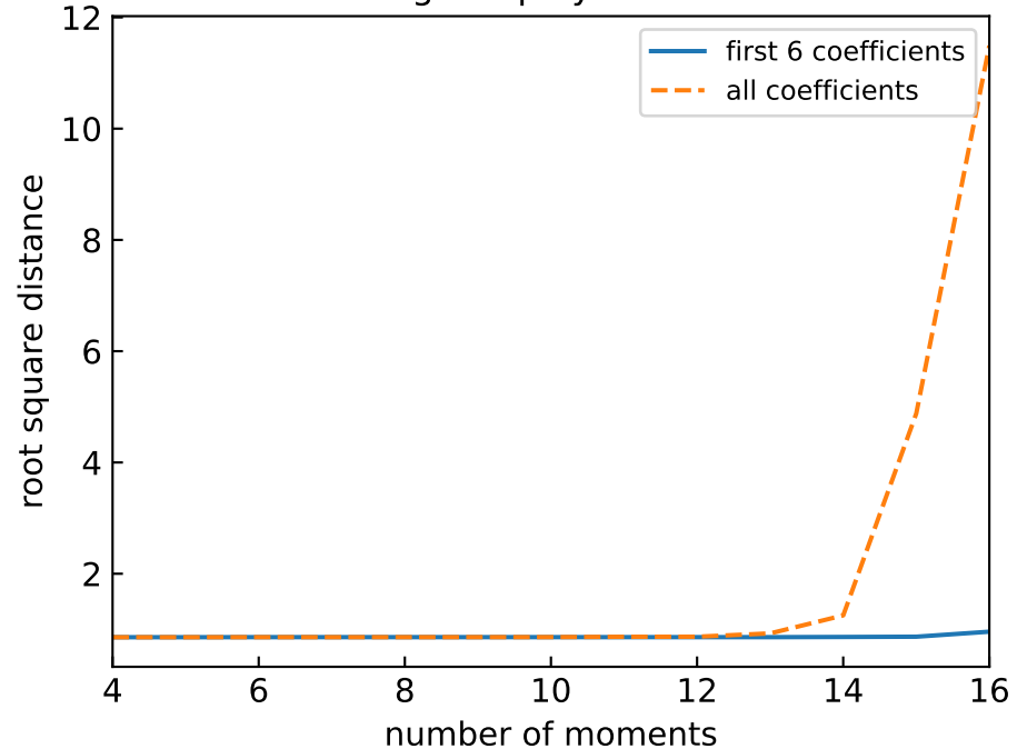
Logistic polynomials
