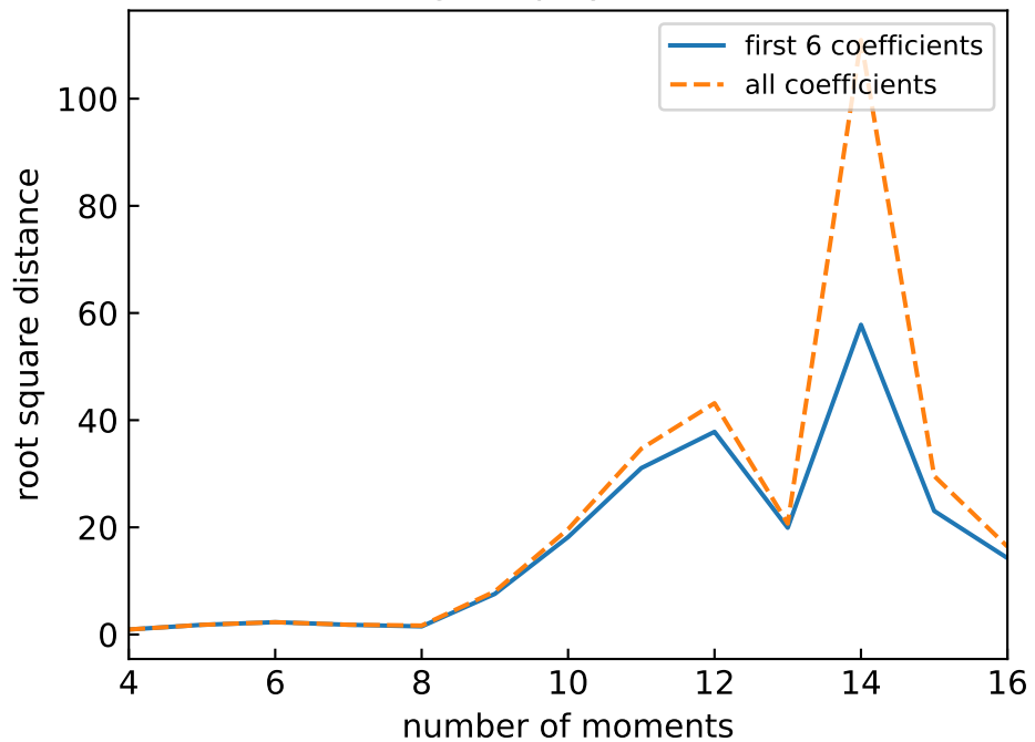
Logistic polynomials
