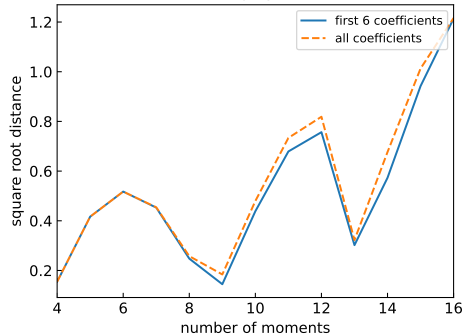
Hermite polynomials
