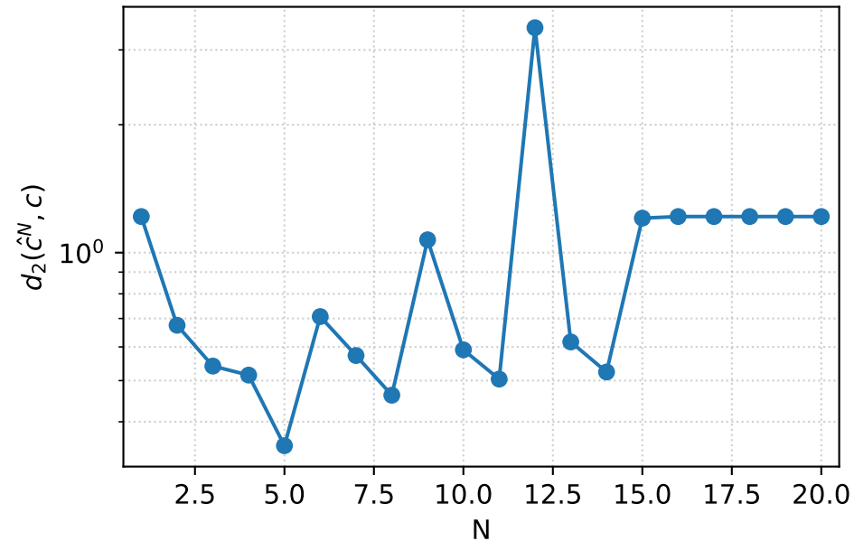
(a) Hermite basis — Heston
