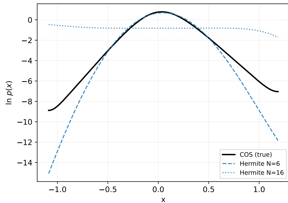
Figure 10: Density comparison — NIG
