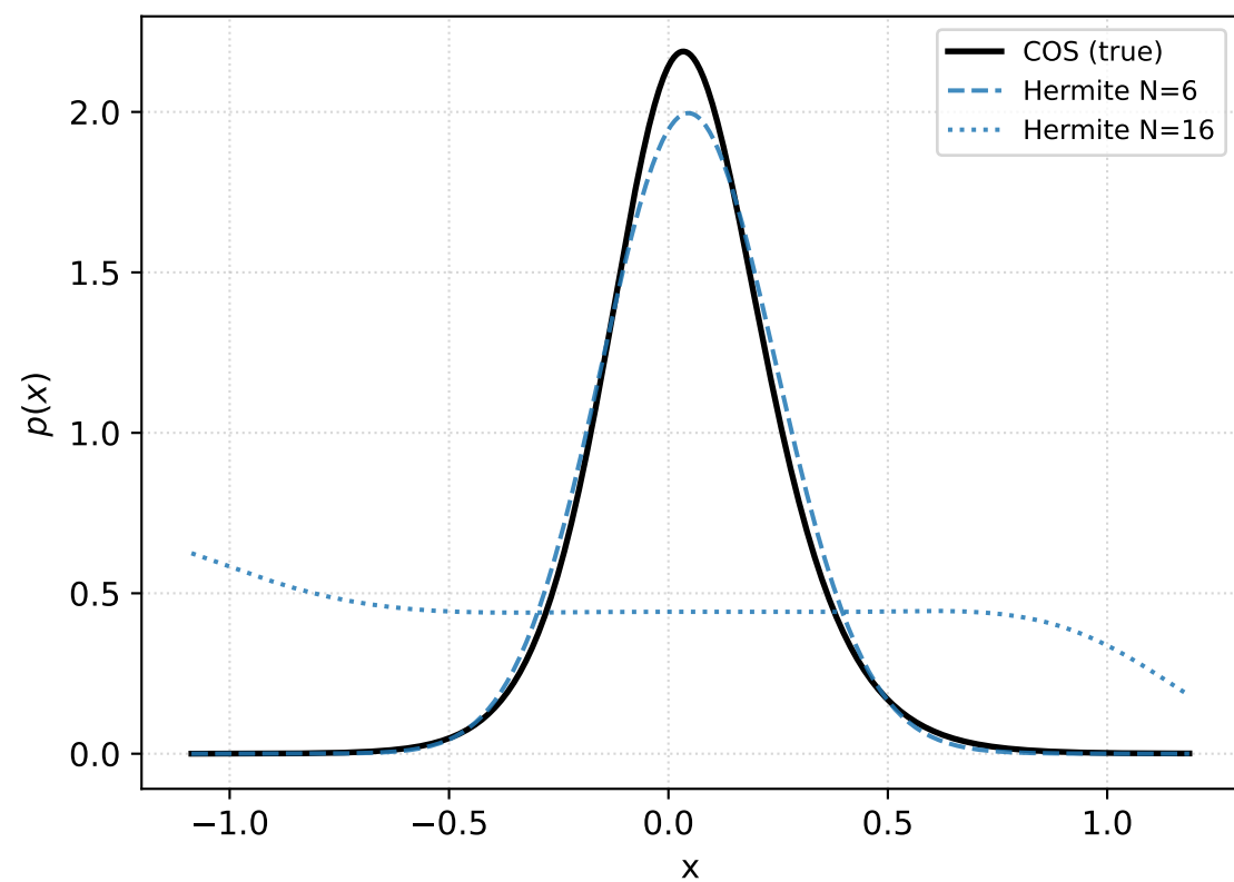
Figure 10: Density comparison — NIG
