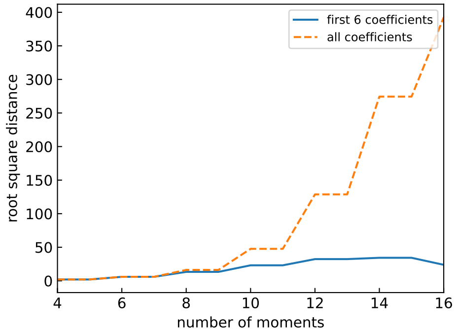
Logistic polynomials
