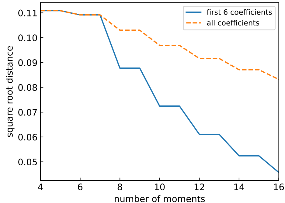
Hermite polynomials
