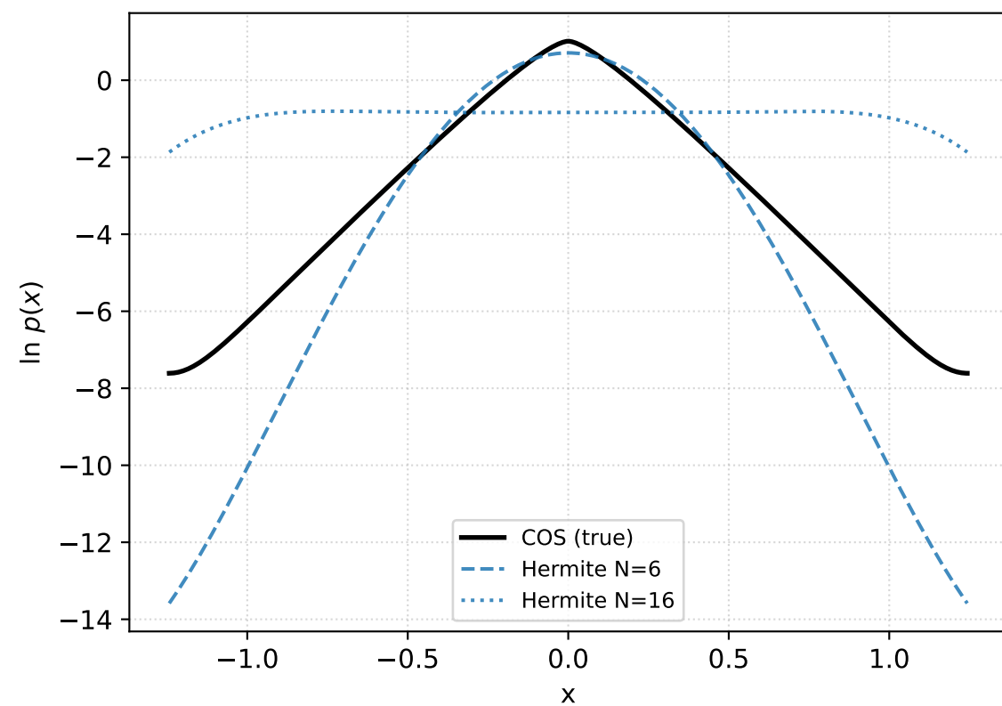
Figure 9: Density comparison — VG
