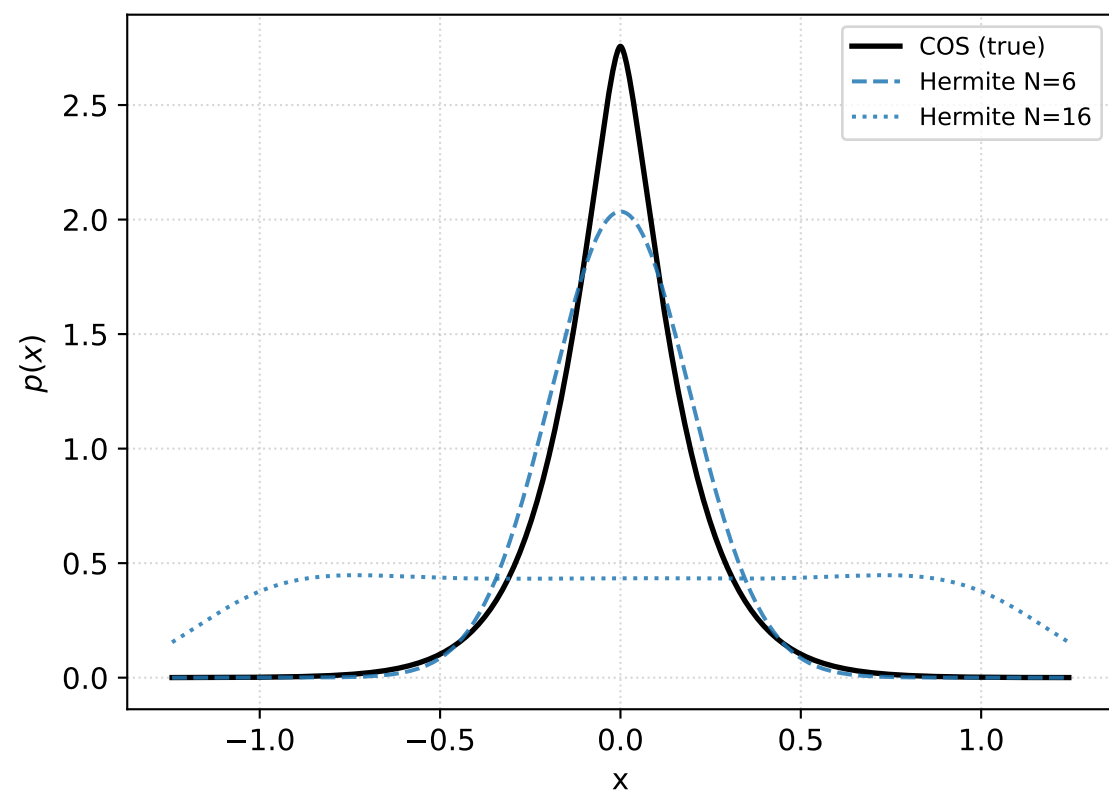
Figure 9: Density comparison — VG
