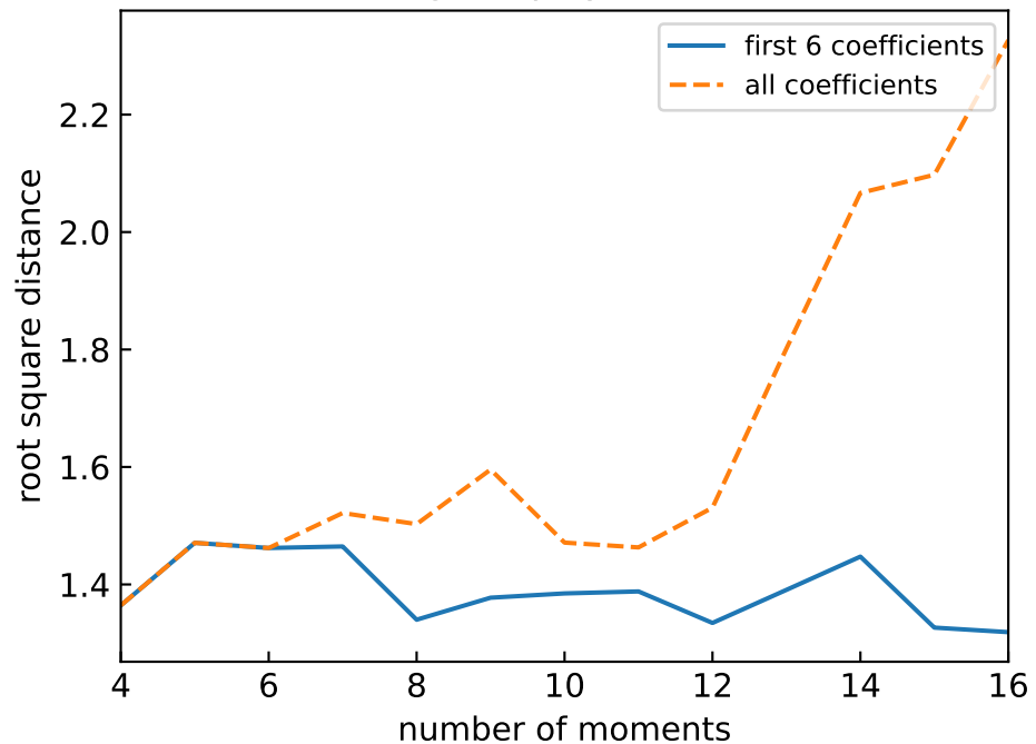
Logistic polynomials
