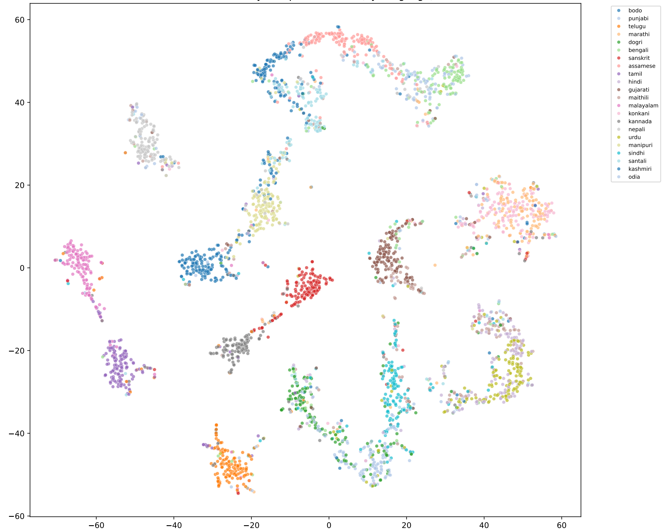
t-SNE of Last Layer Representations (by Language)
