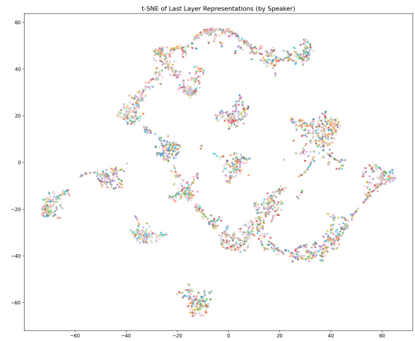
Figure 12: t-SNE visualization of embeddings - colored by speaker (static aug)
