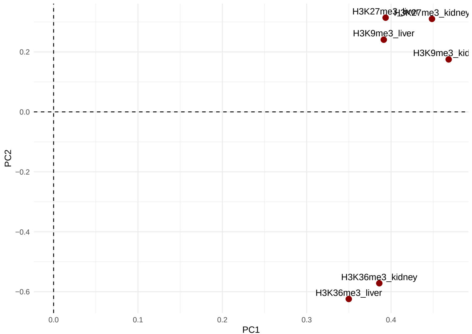
PC1 vs PC2 Loadings
