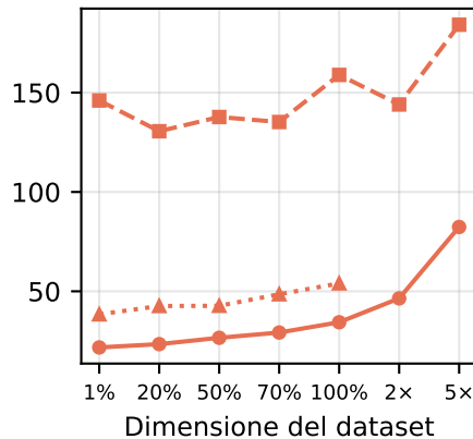
Hive — Job 2
