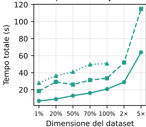
Spark Core — Job 2
