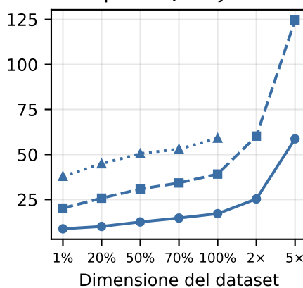
Spark SQL — Job 2
