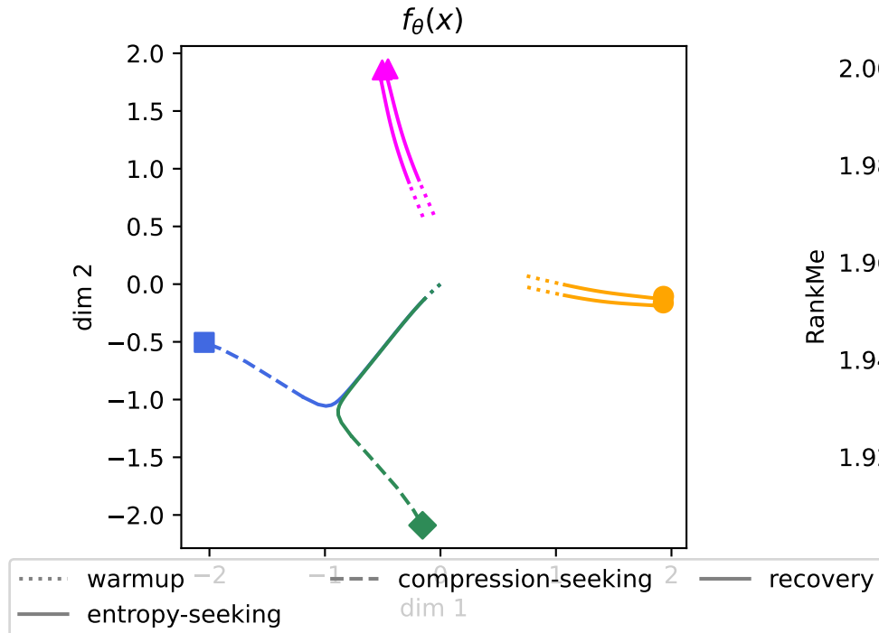
toy single: cross-entropy GD phases
