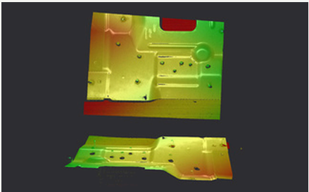
Stamped body panels — two panels in one capture — height map
