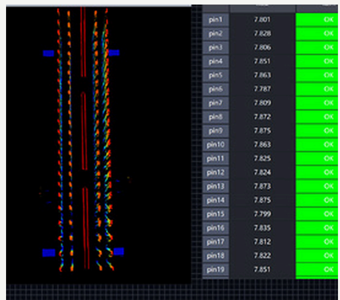
Pin inspection — height of every pin and its pass/fail state in the operator screen
