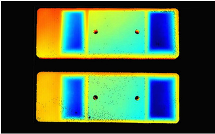
Twin-block railway sleepers — block geometry — height map
