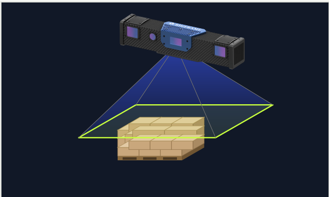
LOGISTICS Depalletizing Layer height and carton positions from one capture at 2.5 m PRS-2500B · VR-2300B Rendering — PRS over a Euro pallet
