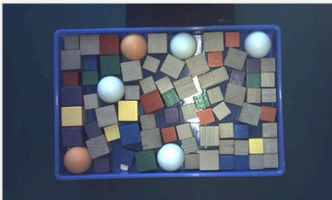
COLLABORATIVE ROBOTS Sorting by color and shape Parts segmented on the registered color image and picked VRD-600B
