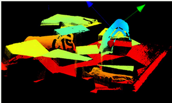
LOGISTICS Parcel singulation and bin picking Grasp points on unsorted parcels from the point cloud VR-600B · VR-1300B · VRD-1200B
