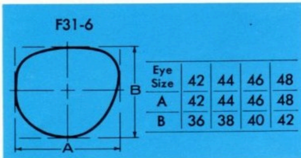
CROSSLEY NUMONT Lens Pattern (6 DIFF.)
