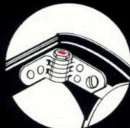
Nylon sleeve compresses against inside of hinge barrel for permanent tightness.
