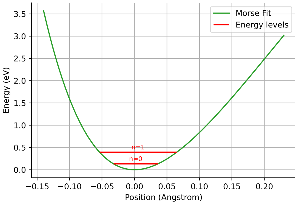
Morse Potential with Energy Levels
