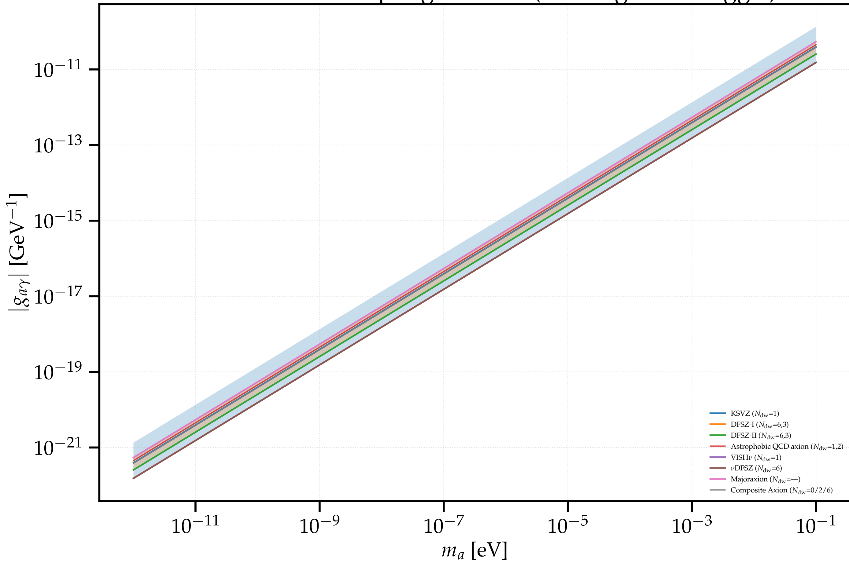
Axion–Photon Coupling vs Mass (click legend to toggle)
