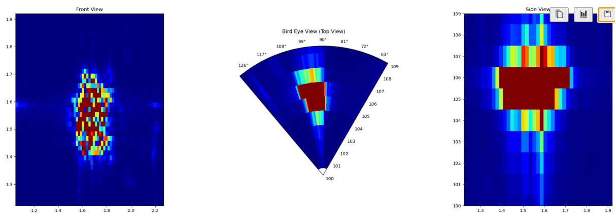
Beamforming 2D example.
