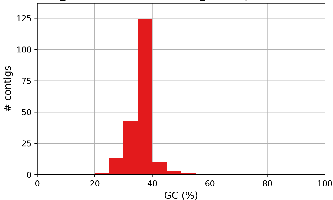
E_faecium.VREN1631.illumina_assembly GC content
