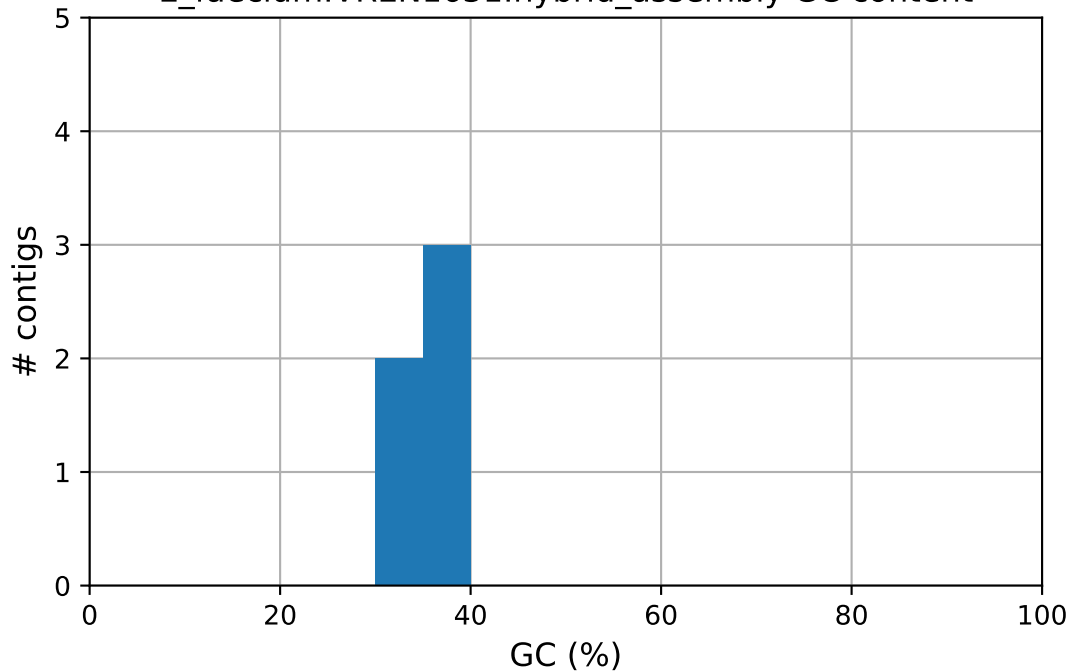
E_faecium.VREN1631.hybrid_assembly GC content
