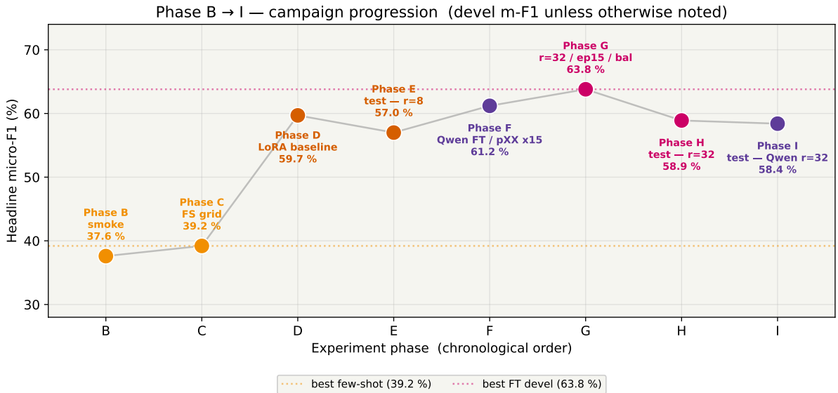
Figure 18: Campaign progression from Phase B (smoke-test, 37.6% devel m-F1) to Phase I (Qwen \times r=32 on test, 58.4%). The two dotted lines show the best few-shot (39.2%) and best fine-tune (63.8%) devel anchors. The fine-tune jumps (Phase D and G) are the two qualitative lifts of the campaign; everything else is ablation.
