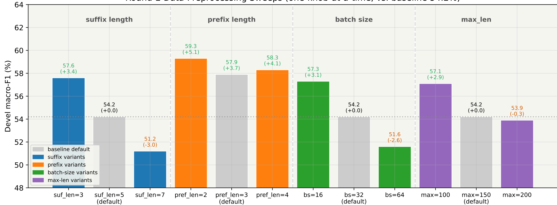
Round-2 Data-Preprocessing Sweeps (one-knob-at-a-time, vs. baseline 54.2%)
