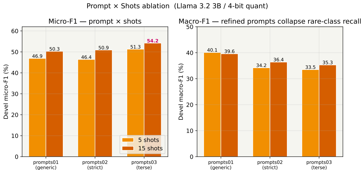
Figure 20: Prompt × shots ablation. Left: micro-F1. Right: macro-F1. The refined prompts ( prompts02 , prompts03 ) trade macro for micro — the best micro ( prompts03 /15 = 54.2% ) has the worst macro (35.3%) because drug_n recall goes to zero. For a rare-class-sensitive task, prompts01 /15 (macro 39.6%) is the saner default.
