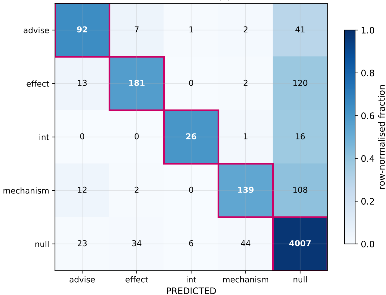
Confusion matrix — mod_best2 single-stage (devel) Recall failures dominate: 29-41% of every positive class leaks to null
