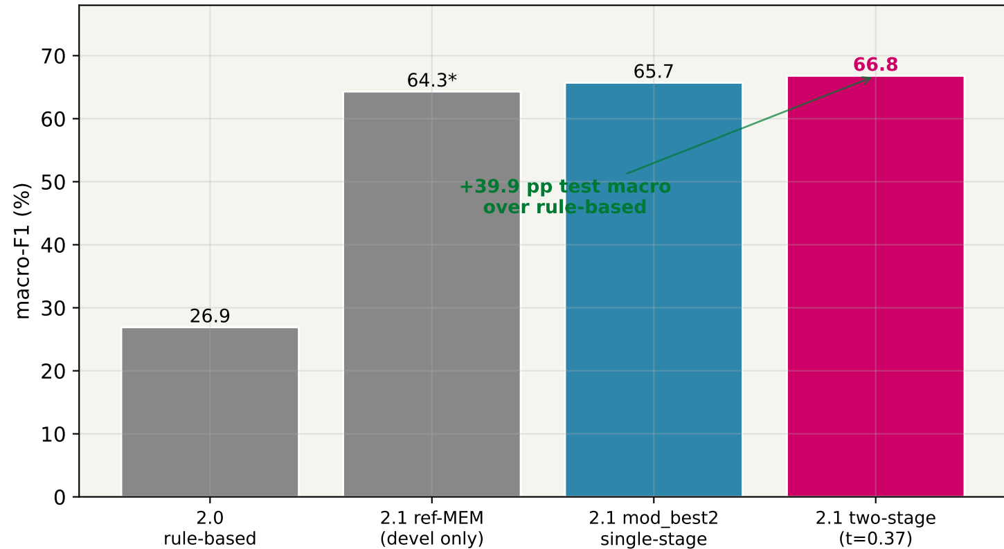
System 2.1 progression (test macro-F1; * = devel-only for ref-MEM)
