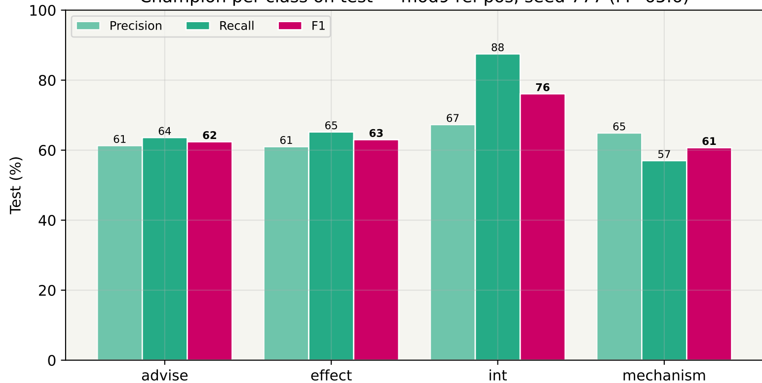
Champion per-class on test — mod9 rel-pos, seed 777 (M=65.6)
