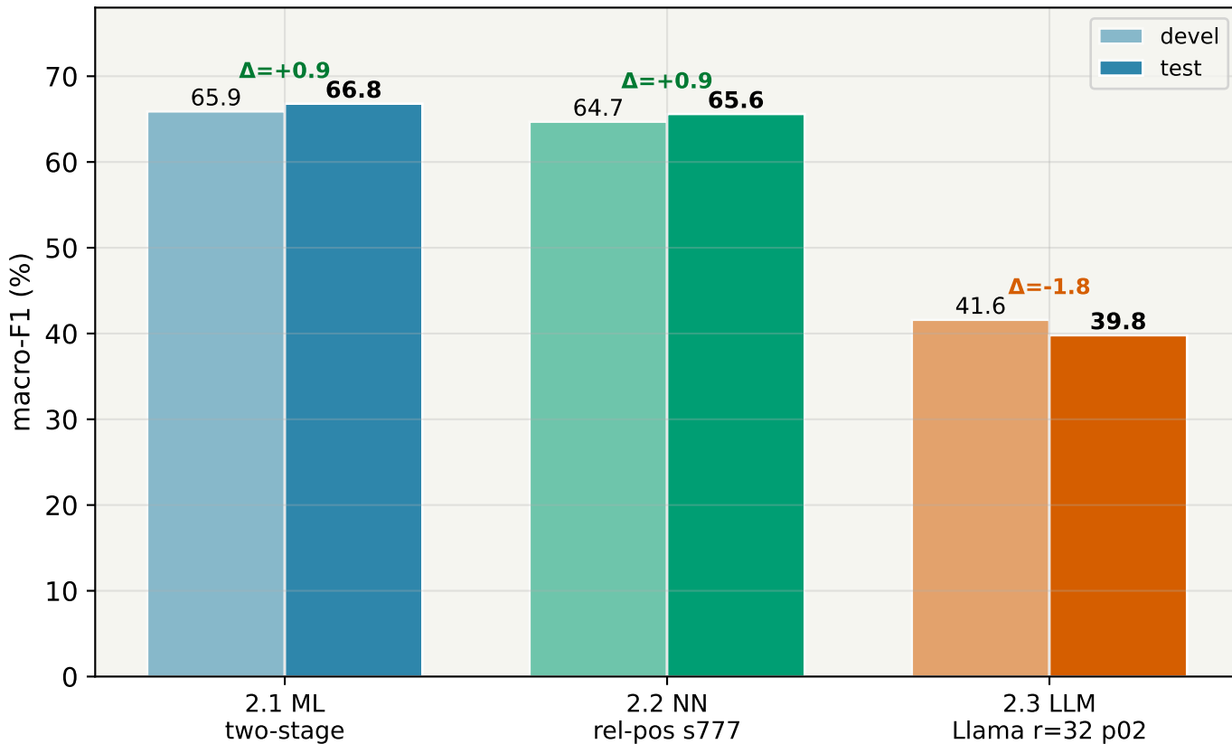
Champion generalisation — devel → test ML & NN generalise positively; the LLM drops slightly but holds rank
