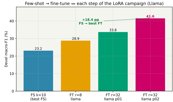
(b) Few-shot \rightarrow fine-tune jump.
