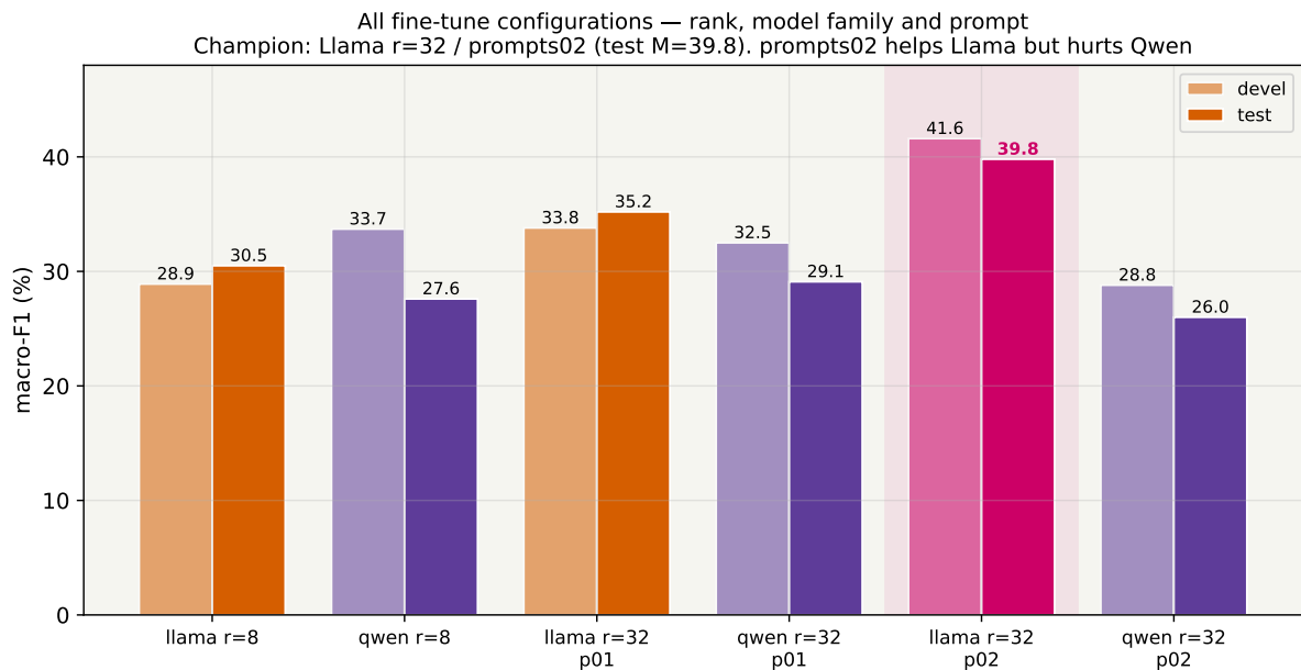
Figure 12: All fine-tune configurations (devel + test macro-F1). LoRA rank 8 \rightarrow 32 and prompt quality are each as powerful as the other — prompt design is a first-class capacity lever, not a free afterthought.
