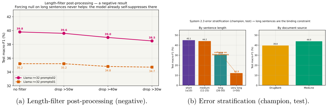
Figure 15: Left: forcing null on long sentences never helps — the collapse there is a recall problem (positives missed), not a precision one a filter could fix. Right: like 2.1 and 2.2, the LLM degrades sharply on long sentences ( M = 12.3 on >50 words), and MedLine is actually slightly easier than DrugBank for the LLM (the opposite of 2.1).
