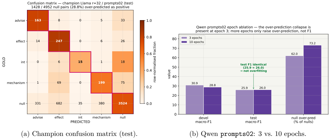
Figure 14: Left: even the champion over-predicts — 28.8 % of all null pairs receive a positive label (precision \ll recall on every class). Right: 3-epoch and 10-epoch Qwen reach identical test F1 (25.9 vs 26.0); more epochs only inflate the over-prediction rate (62%→73%). The collapse is a property of the model×prompt pairing, not of training length.
