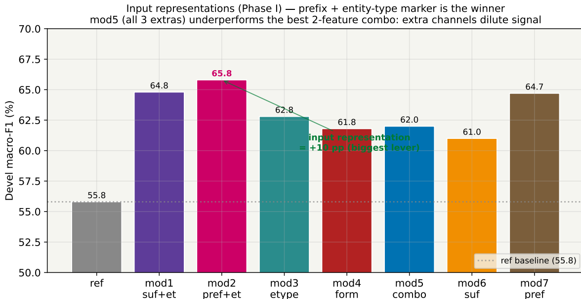
Figure 6: Phase I input-representation sweep. Adding a prefix-3 channel plus an entity-type marker (mod2) lifts macro-F1 by +10 pp over the shipped baseline — the single biggest improvement anywhere in System 2.2.
