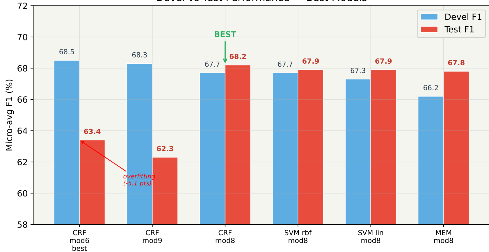
Devel vs Test Performance — Best Models
