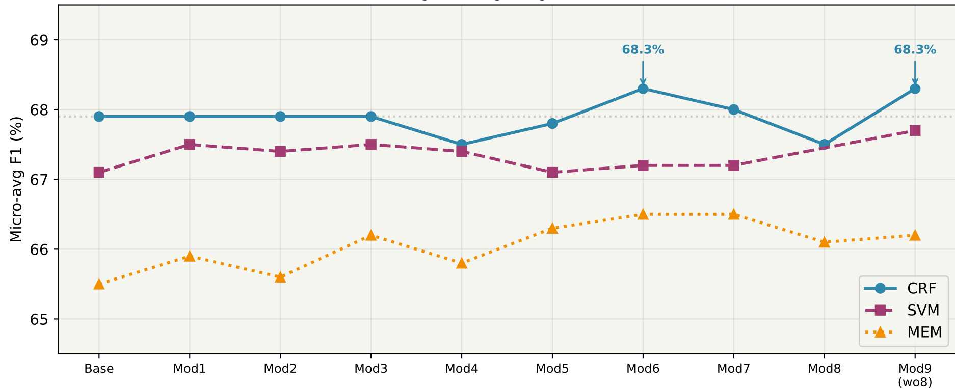
Feature Engineering Progress (Devel Set)
