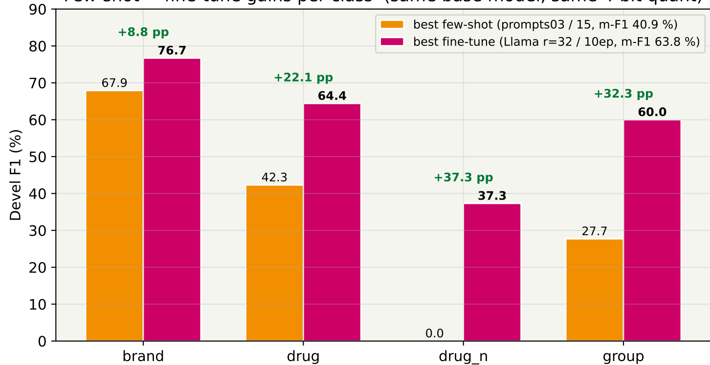
Few-shot → fine-tune gains per class (same base model, same 4-bit quant)
