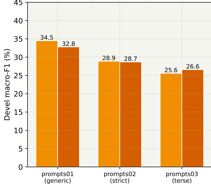
Macro-F1 — refined prompts collapse rare-class recall
