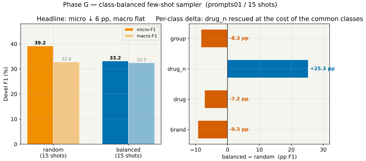
Figure 23: Random vs class-balanced few-shot (prompts01 / 15 shots). Left: headline micro/macro. Right: per-class delta (balanced – random). The balanced sampler lifts drug_n by +25.3pp but loses ground on all three common classes.
