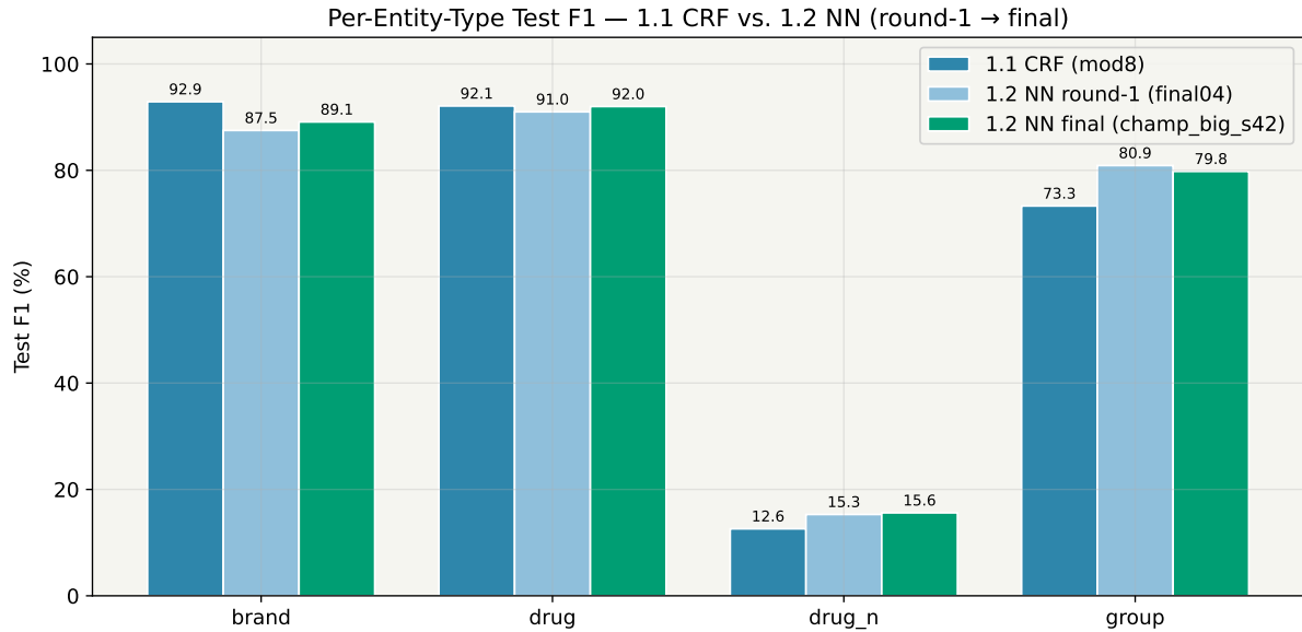
Figure 15: Per-entity-type test F1. The NN system dominates on group (+6.5) and slightly improves on drug_n (+3.0), ties on drug, and loses a few points on brand. The pattern is consistent: the BiLSTM picks up distributional context (which helps semantic classes like group) at the cost of CRF’s sharper local character patterns for trademark-style brand tokens.
