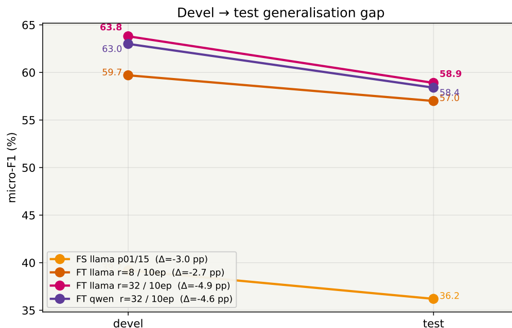
Figure 29: Devel → test generalisation gap. Few-shot’s gap is 3.0 pp; the Phase-D fine-tune’s gap is 2.7 pp; r = 32 ’s gap is 4.9 pp; Qwen+ r = 32 ’s gap is 4.6 pp. The larger adapter overfits devel slightly more, but not enough to lose its test-set lead.
