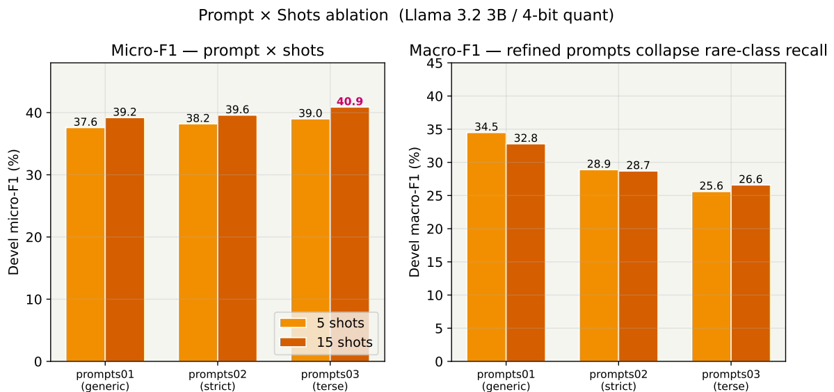
Figure 20: Prompt × shots ablation. Left: micro-F1. Right: macro-F1. The refined prompts ( prompts02 , prompts03 ) trade macro for micro — the best micro ( prompts03/15 = 40.9%) has the worst macro (26.6%) because drug_n recall goes to zero. For a rare-class-sensitive task, prompts01/15 (macro 32.8%) is the saner default.
