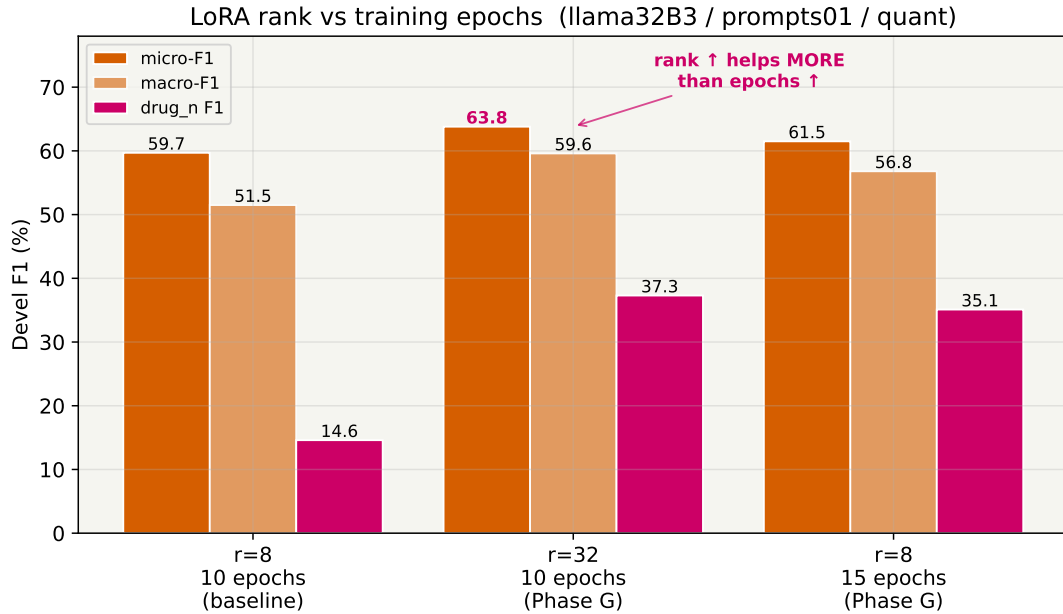
Figure 22: LoRA rank vs training epochs (Llama, 4-bit, prompts01 ). Quadrupling rank ( r = 8 \rightarrow r = 32 , \alpha = 16 \rightarrow \alpha = 64 ) lifts micro-F1 by +4.1 pp and macro-F1 by +8.1 pp over the Phase-D baseline. Adding five more training epochs (15 vs 10) lifts micro-F1 by only +1.8 pp . Rank capacity matters more than training time.
