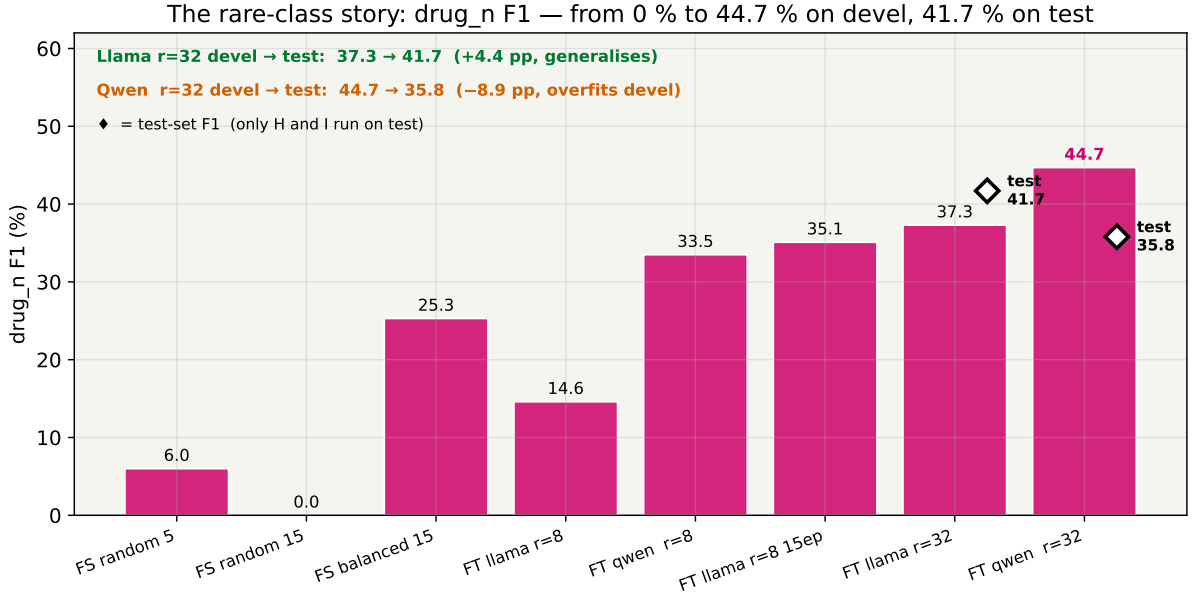
Figure 25: The drug_n rare-class story across the campaign. Bars are devel F1; diamonds are test-set F1 for the two test-run fine-tune configurations. The Qwen overfit on devel (44.7% devel → 35.8% test) is the single biggest surprise of Phase I; Llama holds (and slightly improves) under the same split change.
