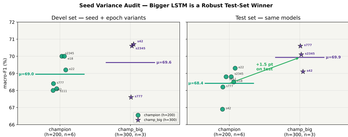
Figure 13: Seed variance on devel (left) and test (right) for the two architectures. Horizontal lines are the means. On test, every champ_big run beats the champion mean (68.4), and the champ_big mean (69.9) beats the best single champion run (69.3) — a +1.5 point mean-over-mean improvement that survives seed variance, though the per-run ranges overlap slightly.
