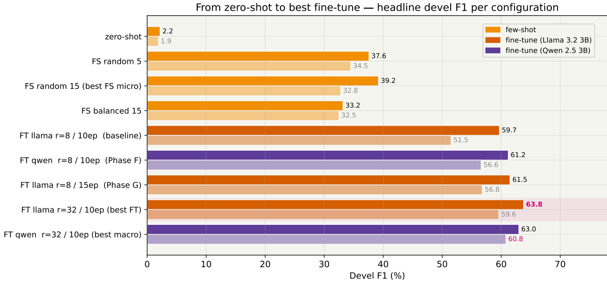
Figure 26: Headline devel F1 across all nine flagship configurations, from zero-shot (2.2%) to the best fine-tune (63.8%). Lighter bars are macro-F1 shadows. The pink highlight marks the single best-micro configuration.
