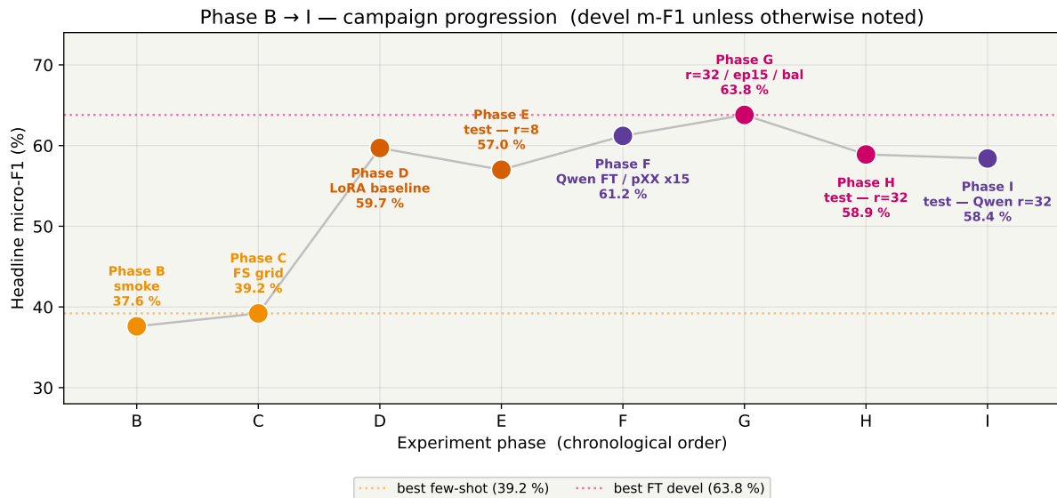
Figure 18: Campaign progression from Phase B (smoke-test, 37.6% devel m-F1) to Phase I (Qwen×r=32 on test, 58.4%). The two dotted lines show the best few-shot (39.2%) and best fine-tune (63.8%) devel anchors. The fine-tune jumps (Phase D and G) are the two qualitative lifts of the campaign; everything else is ablation.
