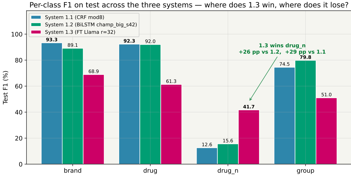
Figure 32: Per-class test F1 across the three systems. The LLM only wins one column ( drug_n , the rare class) but does so by a very large margin. On the three common classes, the CRF’s sharp character-level patterns and the BiLSTM’s learned embeddings dominate by 20–30 pp.
