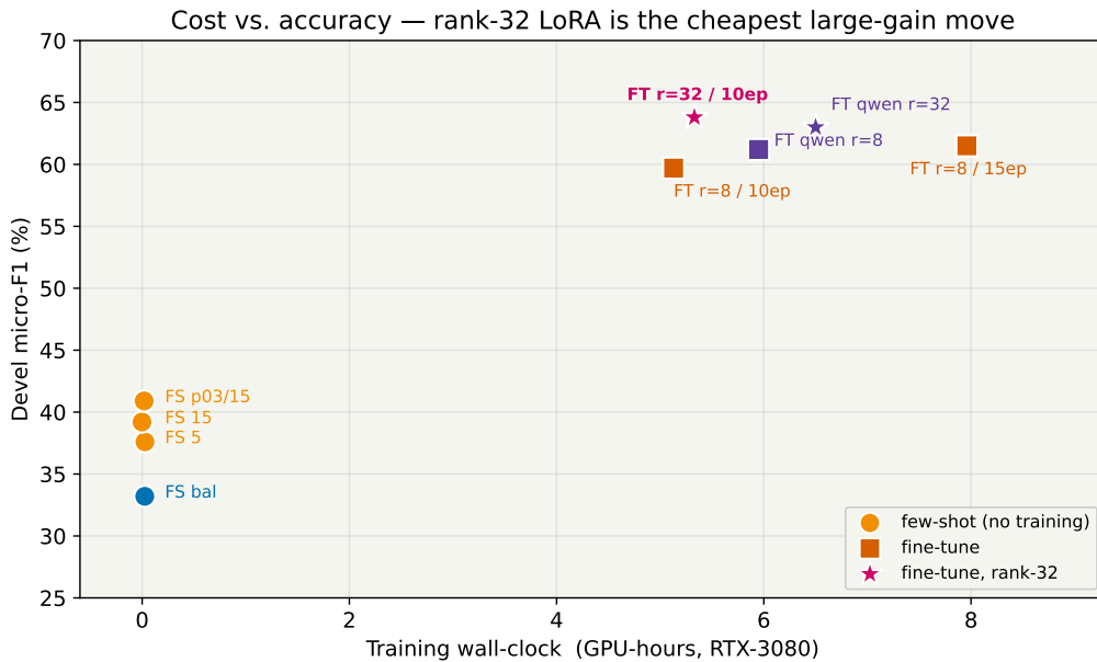
Figure 27: GPU-hours vs devel micro-F1. Few-shot is free but capped around 40%. Fine-tuning at r = 32 (stars) is the cheapest way to reach the 63% regime; 15 epochs at r = 8 is both slower and weaker.
