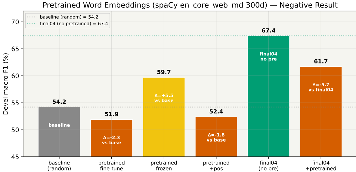
Figure 11: Pretrained word embeddings on the lower-cased-word channel. Fine-tuning destroys the pretrained structure ( -2.3 vs. random); freezing partially recovers ( +5.5 ); stacking pretrained vectors on top of final04 drops macro-F1 by -5.7 . spaCy md is trained on generic news text and carries the wrong priors for drug names.
