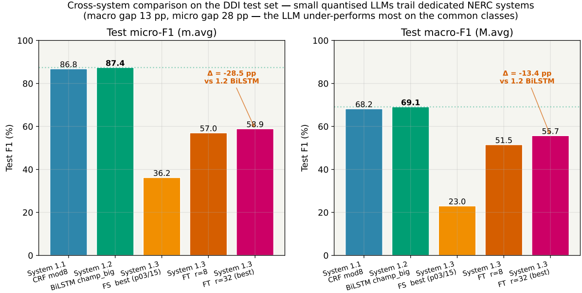
Figure 31: Cross-system headline comparison on the DDI test set. Left: micro-F1 (m.avg). Right: macro-F1 (M.avg). The best System 1.3 system (FT Llama r = 32 ) trails System 1.2 by -28.5 pp on micro and -13.4 pp on macro. The gap is smaller on macro — the LLM is comparatively more competitive on the harder classes than on the easy ones.
