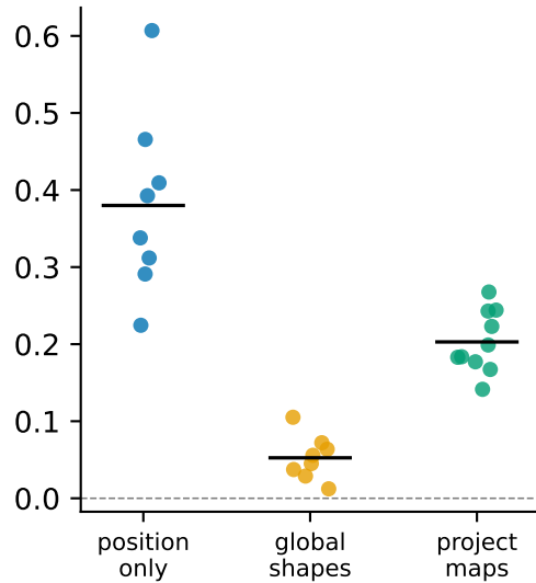
gain over shuffled layout
