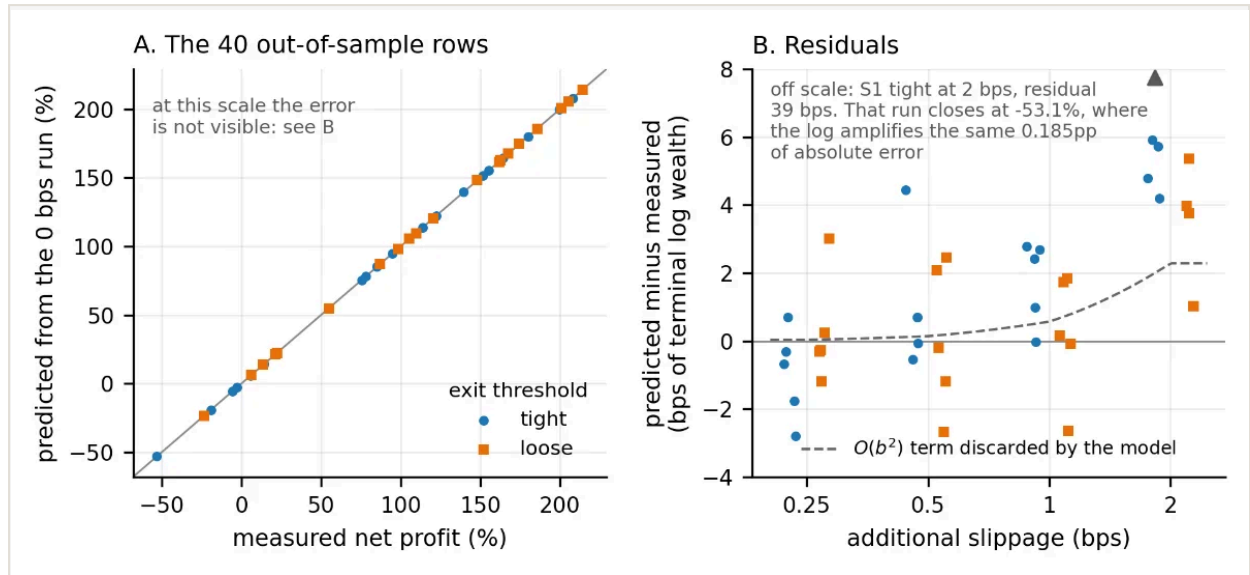
F1. Out-of-sample validation of the cost reconstruction
