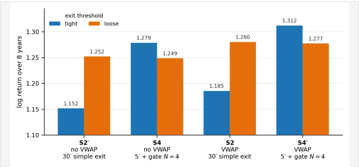
F2. The four cells of the VWAP entry filter × exit structure plane, under the two exit thresholds
