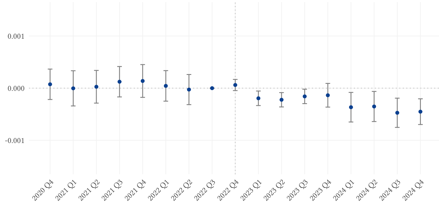
Spillover Analysis: Texas
