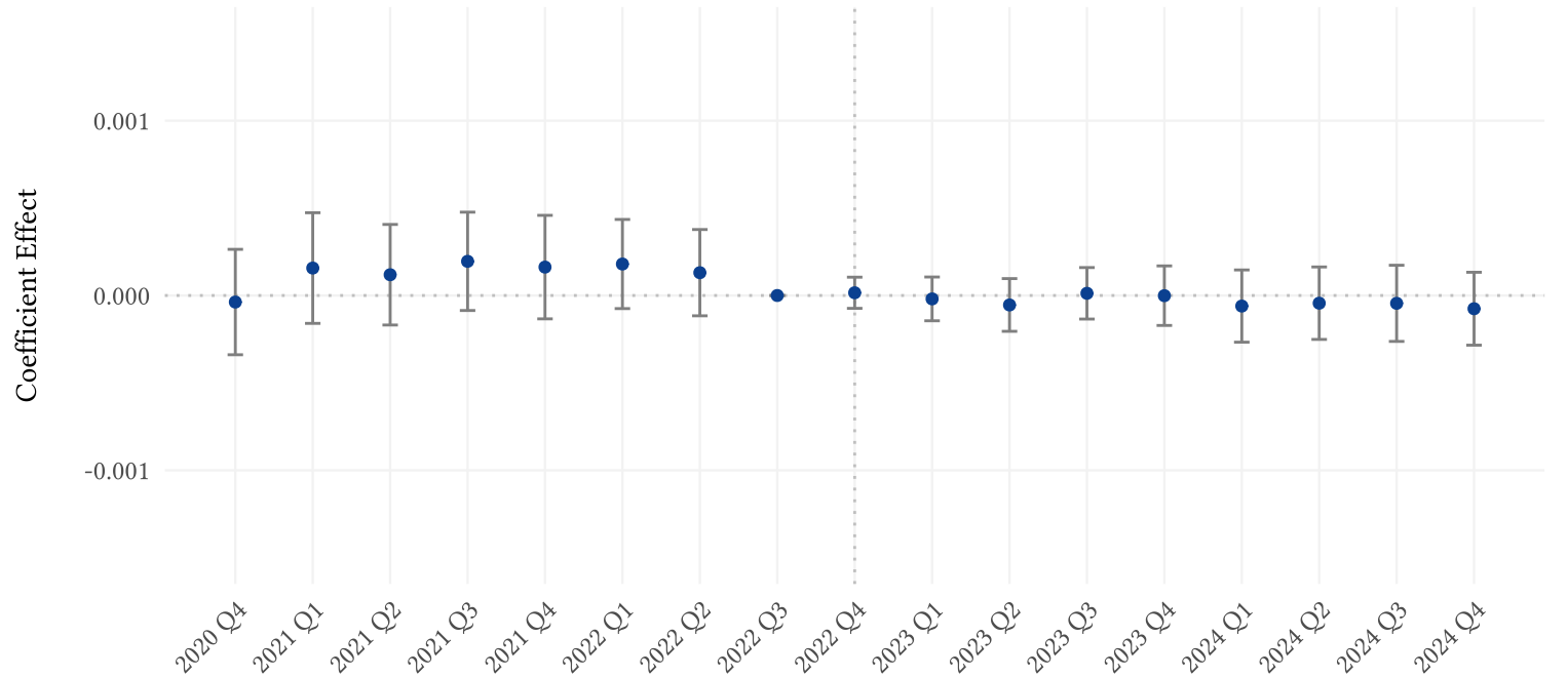
Spillover Analysis: California
