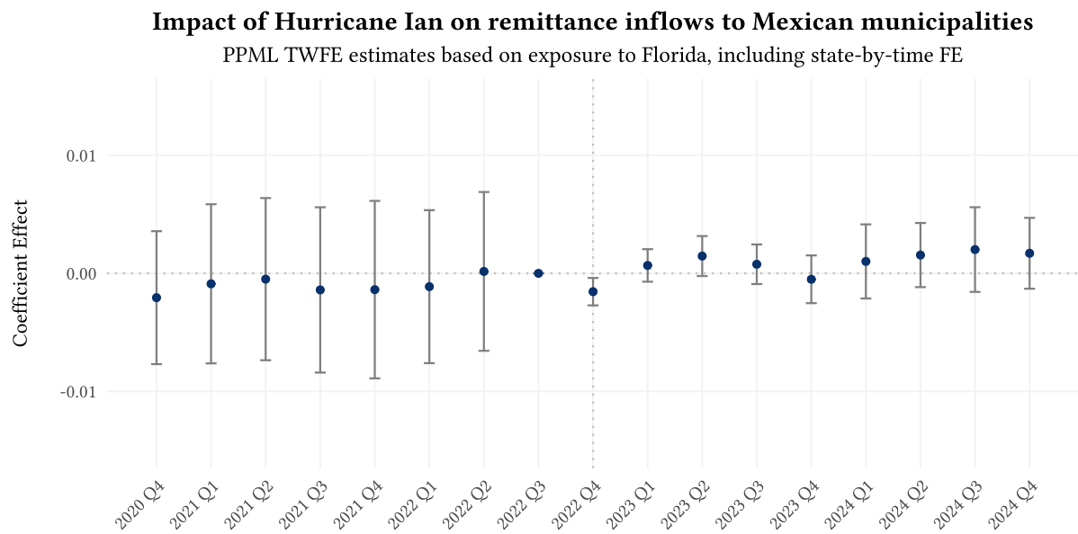
Figure 4.2: PPML Event Study Estimates
