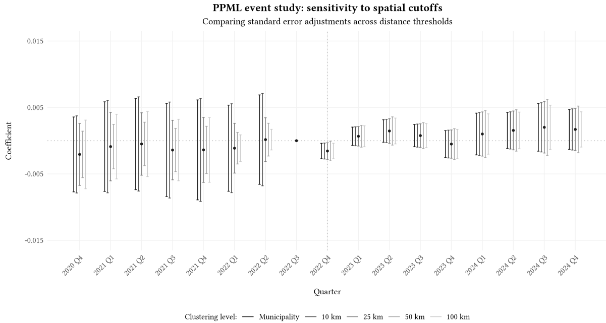
Figure 4.3: PPML Event Study Estimates with Conley Standard Errors for Different Buffer Distances
