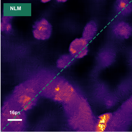
Non-Local Means
