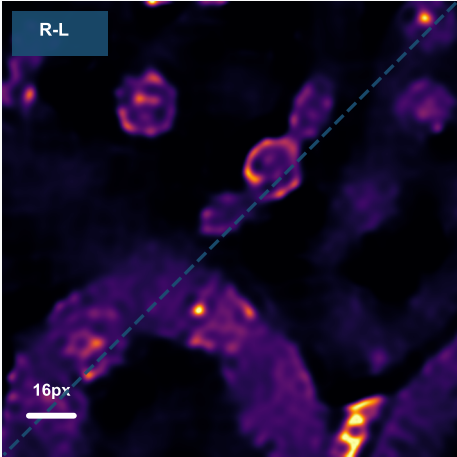
Richardson–Lucy
