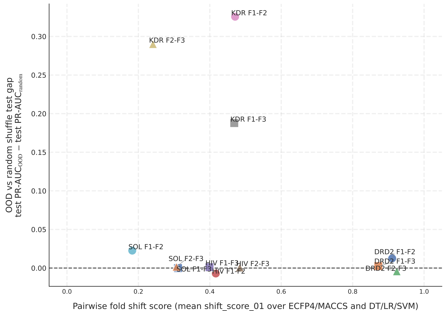
Pairwise fold shift vs protocol-selection benefit on OOD test
