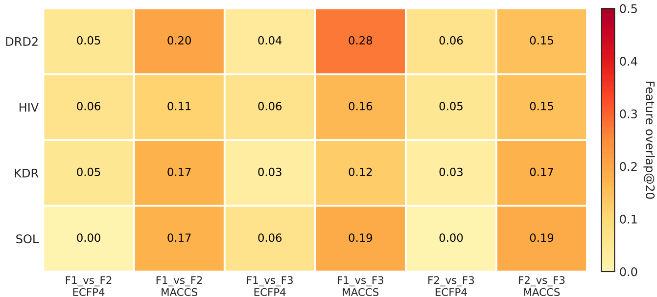
Activity features (List A) vs Shift features (List B): top-20 overlap
