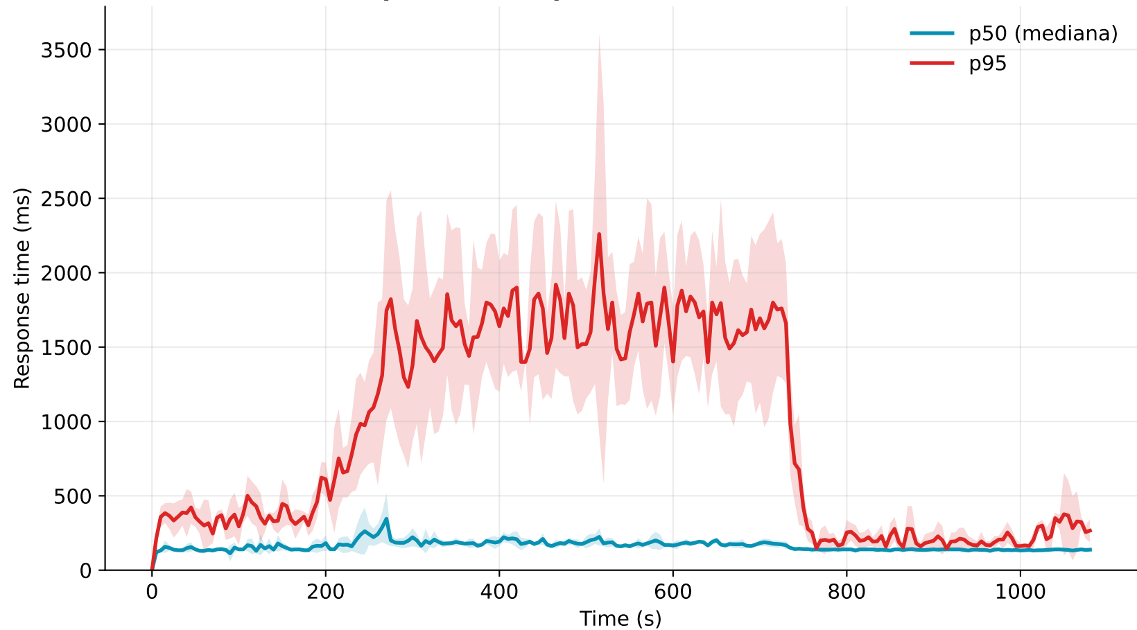
Response time (percentiles) — Continuous
