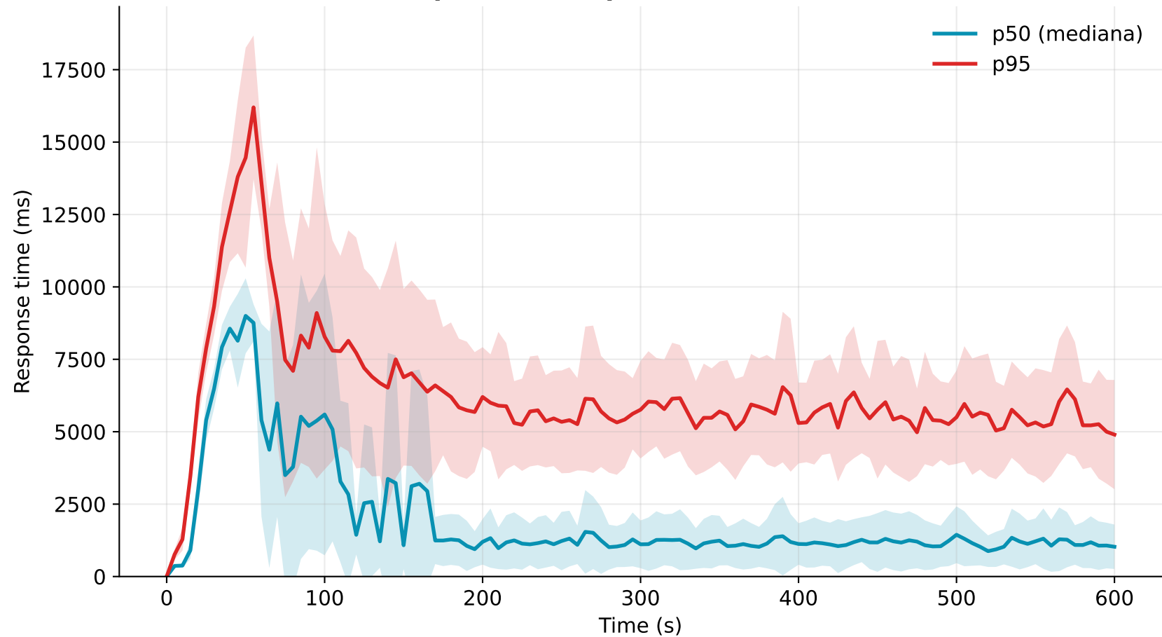
Response time (percentiles) — Stress
