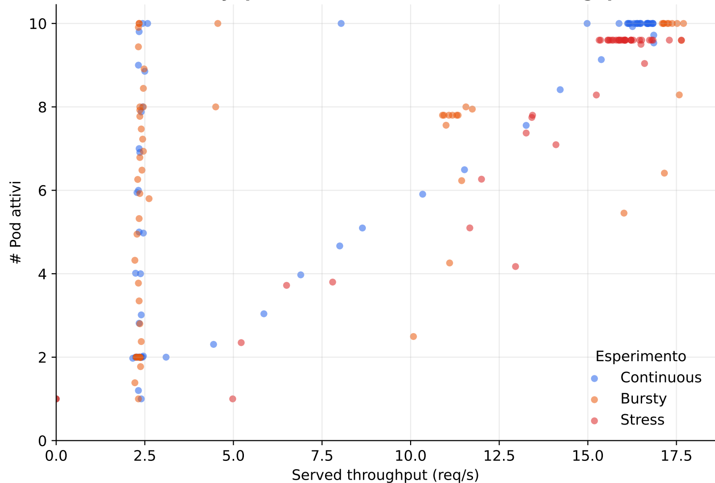
Scalability: pods needed as a function of throughput
