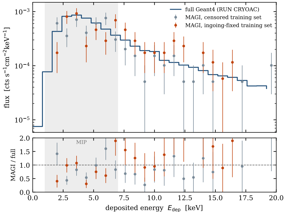
CR – SRON XFDM, Detector 1 (TES array)
