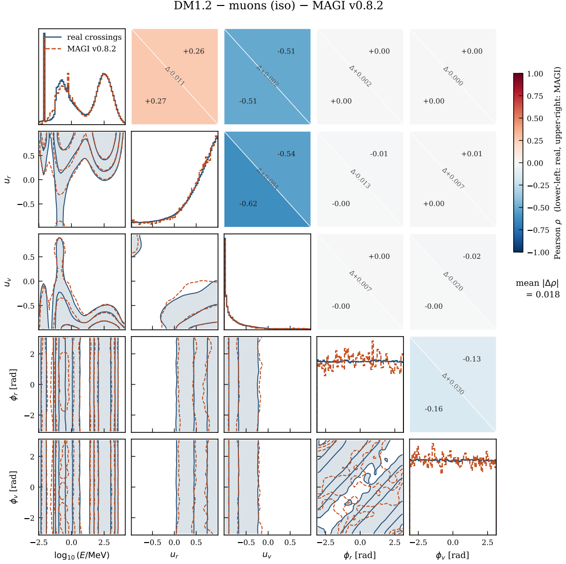
Figure 2: Figure 2 candidate — DM1.2 (recommended). Crossing population, real vs MAGI. Lower triangle: 2D contours. Diagonal: marginals. Upper triangle: each cell split diagonally, lower-left half the real Pearson \rho , upper-right half MAGI's, on a common scale with the residual printed — a visually uniform cell is a reproduced correlation.
